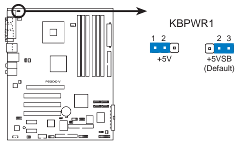
P5GDC-V Keyboard power setting
