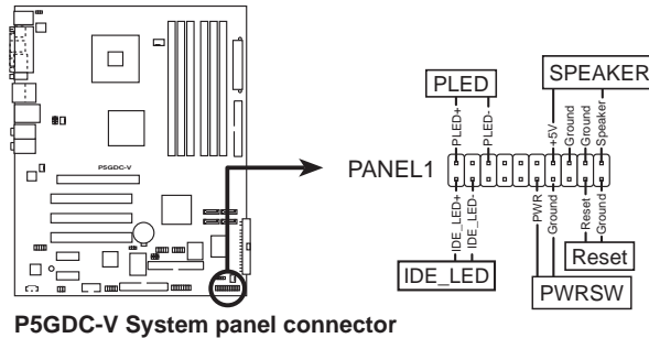
P5GDC-V System panel connector
