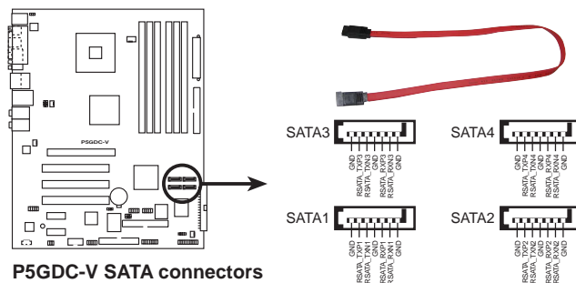
P5GDC-V SATA connectors
